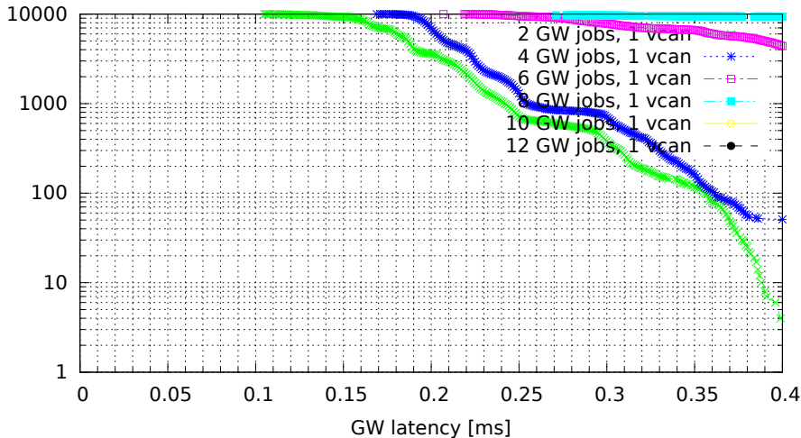
Chained GWs on a single VCAN interface (GW kernel 2.6.33.7-rt29-00004-g92487e4, Traffic 50, Load none)
