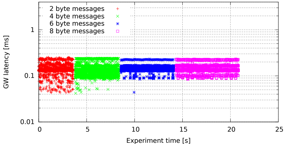
Single GW rule for all messages, no modifications, high (soft)irq task priority (GW kernel 2.6.33.7-rt29-00004-g92487e4, Traffic 50, Load none)
