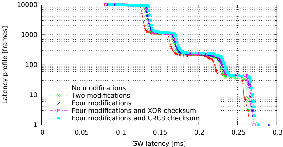
Single GW rule for all messages with modifications, 8 byte messages (GW kernel 2.6.33.7-rt29-00004-g92487e4, Traffic 50, Load none)
