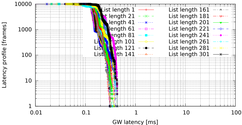
Different lengths of filter list, only the last one matches (GW kernel 2.6.33.7-rt29-00004-g92487e4, Traffic 50, Load none)
