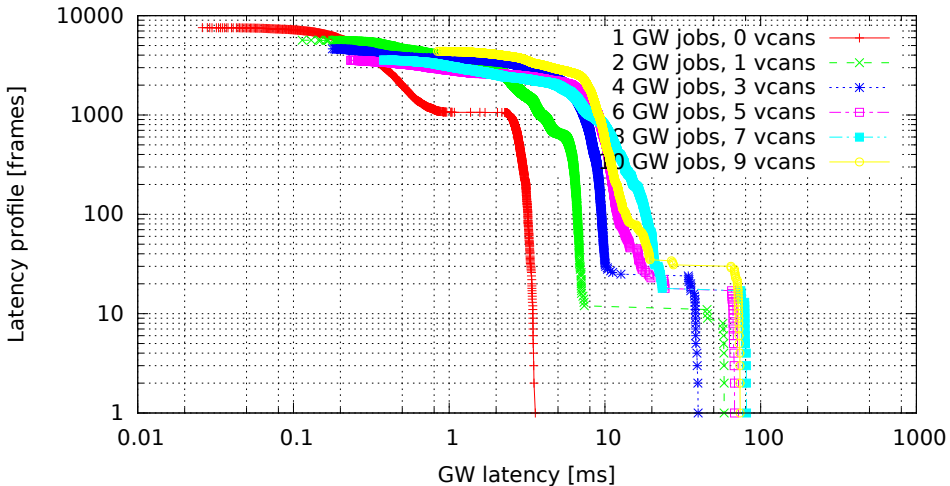
Chained GWs on multiple VCAN interfaces (GW kernel 2.6.33.7-rt29-00004-g92487e4, Traffic 50, Load eth)
