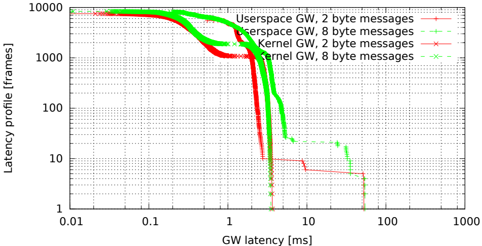
Kernel vs. userspace GW, no modifications (GW kernel 2.6.33.7-rt29-00004-g92487e4, Traffic 50, Load eth)
