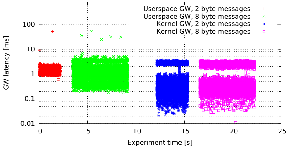
Single GW rule for all messages, no modifications (GW kernel 2.6.33.7-rt29-00004-g92487e4, Traffic 50, Load eth)
