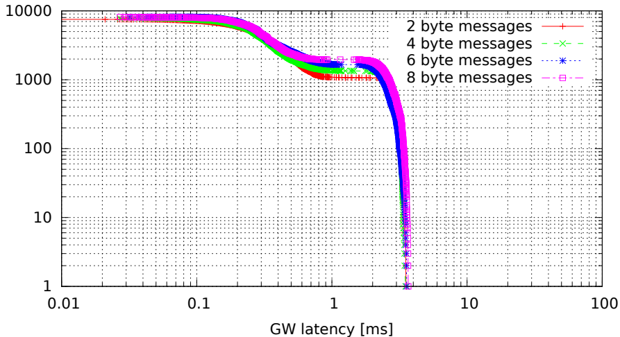
Single GW rule for all messages, no modifications (GW kernel 2.6.33.7-rt29-00004-g92487e4, Traffic 50, Load eth)
