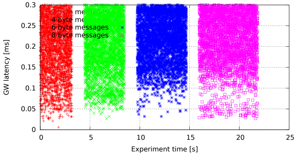
Single GW rule for all messages, no modifications (GW kernel 2.6.33.7-rt29-00004-g92487e4, Traffic 50, Load eth)
