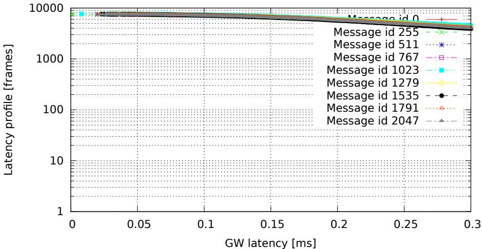
2048 GW rules (one per id, mask C00007FF), no modifications (GW kernel 2.6.33.7-rt29-00004-g92487e4, Traffic 50, Load eth)
