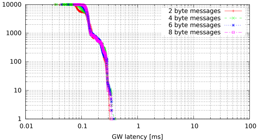
Single GW rule for all messages, no modifications (GW kernel 2.6.33.7-rt29-00004-g92487e4, Traffic 50, Load cpu)
