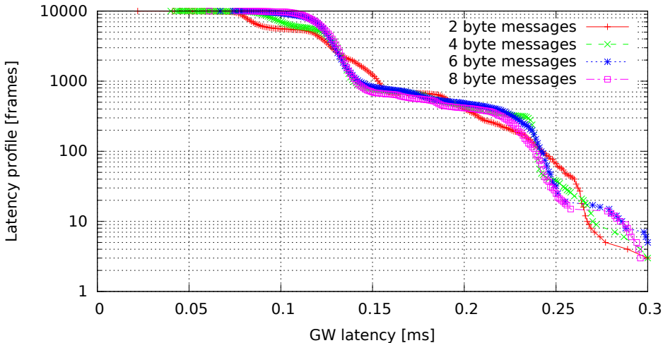
Single GW rule for all messages, no modifications, high (soft)irq task priority (GW kernel 2.6.33.7-rt29-00004-g92487e4, Traffic 50, Load cpu)
