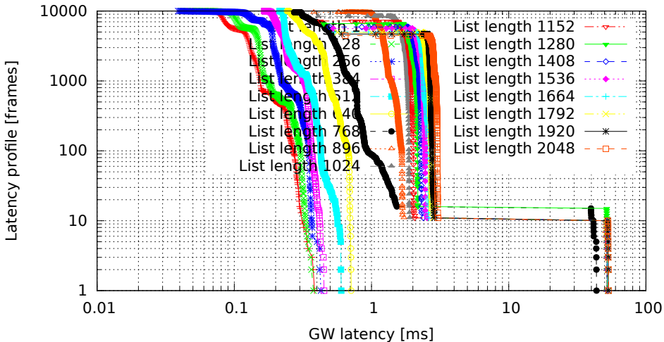
Different lengths of filter list, only the last one matches (GW kernel 2.6.33.7-rt29-00004-g92487e4, Traffic 50, Load cpu)
