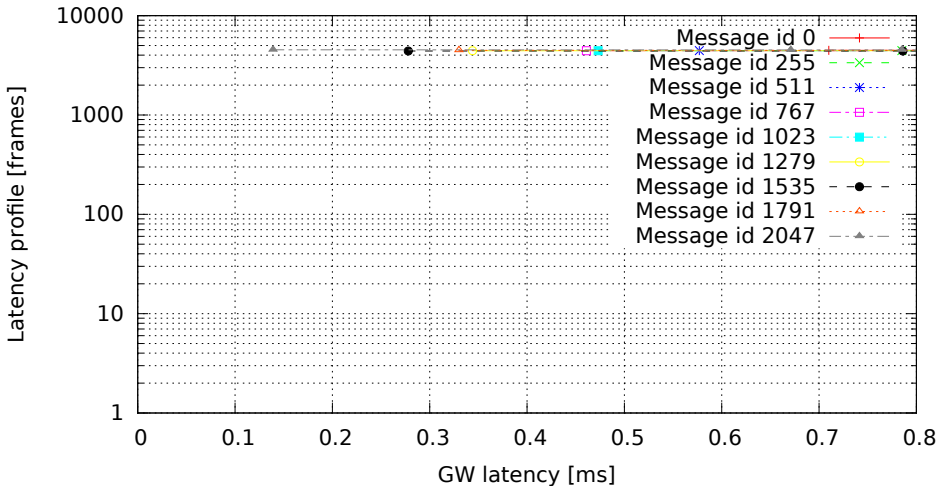
2048 GW rules (one per id, mask 0x7FF), no modifications (GW kernel 2.6.33.7-rt29-00004-g92487e4, Traffic 50, Load cpu)
