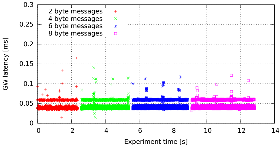
Single GW rule for all messages, no modifications, high (soft)irq task priority (GW kernel 2.6.33.7-00007-g9c0ff90, Traffic oneatatime, Load none)
