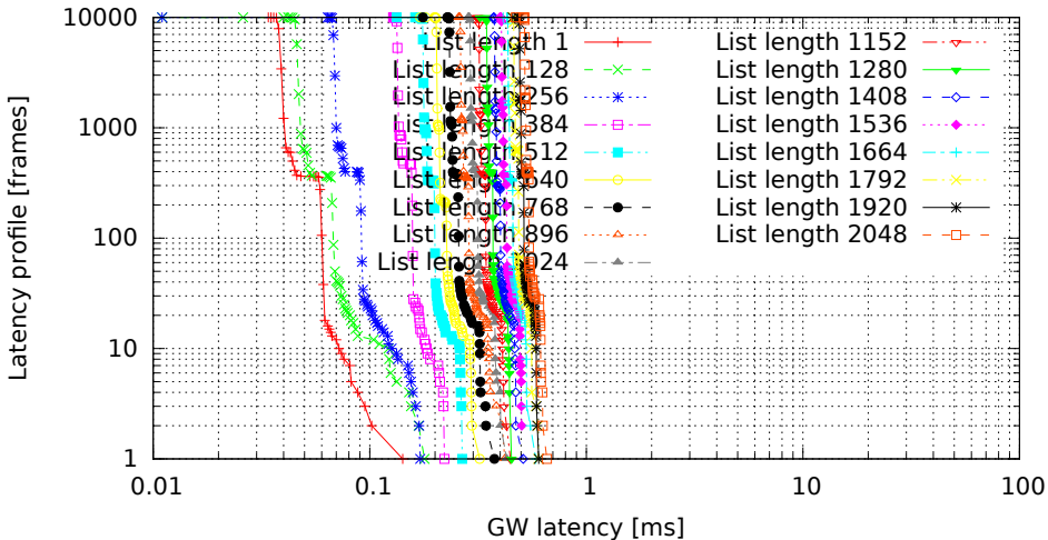
Different lengths of filter list, only the last one matches (GW kernel 2.6.33.7-00007-g9c0ff90, Traffic oneatatime, Load none)
