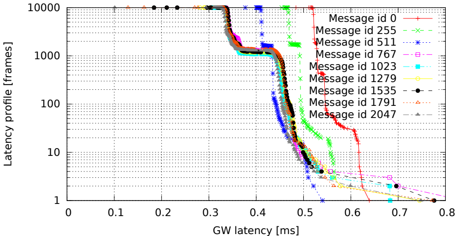
2048 GW rules (one per id, mask 0x7FF), no modifications (GW kernel 2.6.33.7-00007-g9c0ff90, Traffic onetatime, Load none)
