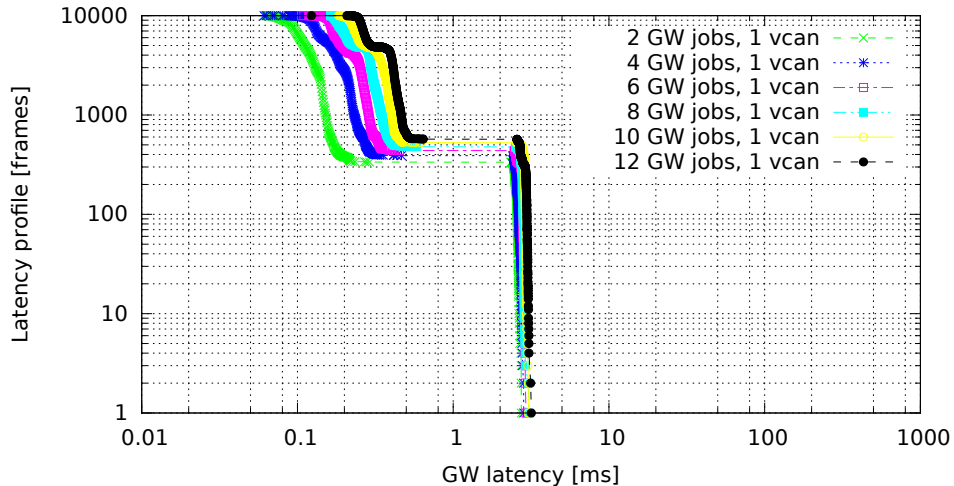
Chained GWs on a single VCAN interface (GW kernel 2.6.33.7-00007-g9c0ff90, Traffic oneatatime, Load eth)
