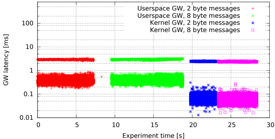
Single GW rule for all messages, no modifications (GW kernel 2.6.33.7-00007-g9c0ff90, Traffic onetotime, Load eth)
