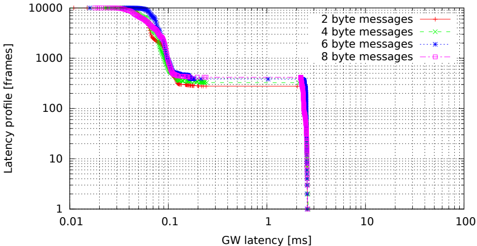
Single GW rule for all messages, no modifications (GW kernel 2.6.33.7-00007-g9c0ff90, Traffic oneatatime, Load eth)
