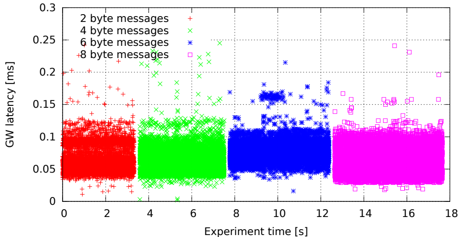
Single GW rule for all messages, no modifications (GW kernel 2.6.33.7-00007-g9c0ff90, Traffic onetatime, Load eth)
