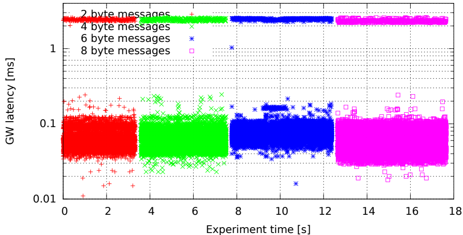
Single GW rule for all messages, no modifications (GW kernel 2.6.33.7-00007-g9c0ff90, Traffic oneatatime, Load eth)
