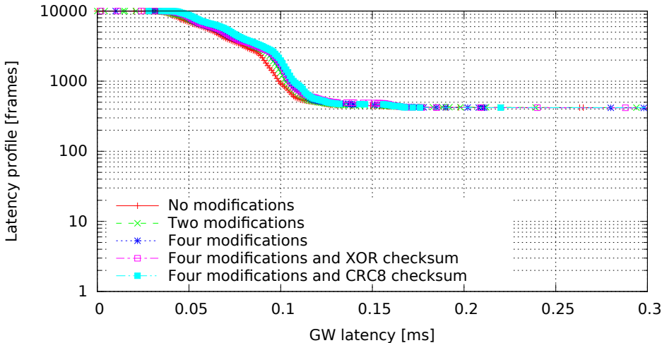
Single GW rule for all messages with modifications, 8 byte messages (GW kernel 2.6.33.7-00007-g9c0ff90, Traffic oneatatime, Load eth)
