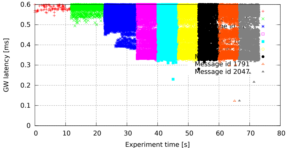
2048 GW rules (one per id, mask 0x7FF), no modifications (GW kernel 2.6.33.7-00007-g9c0ff90, Traffic oneatatime, Load eth)
