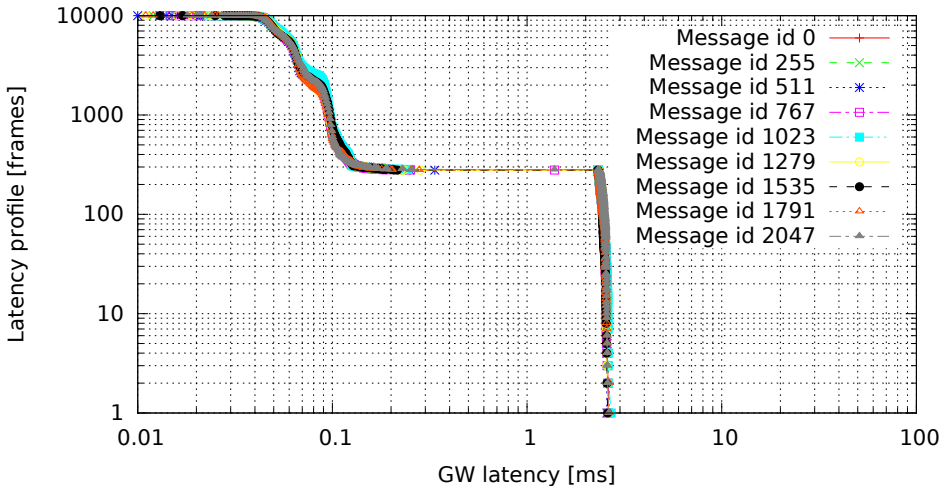
2048 GW rules (one per id, mask C00007FF), no modifications (GW kernel 2.6.33.7-00007-g9c0ff90, Traffic oneatatime, Load eth)
