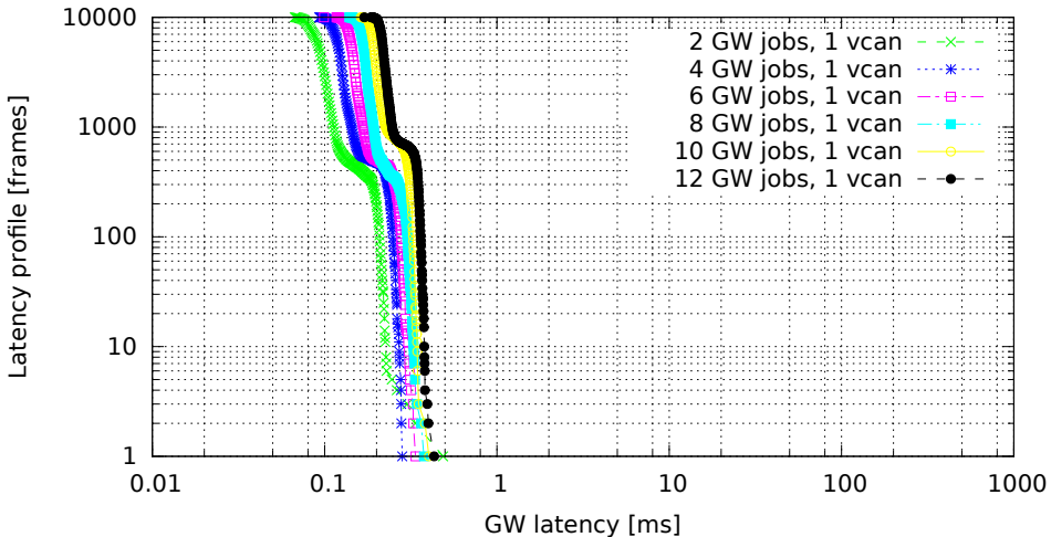
Chained GWs on a single VCAN interface (GW kernel 2.6.33.7-00007-g9c0ff90, Traffic oneatatime, Load cpu)
