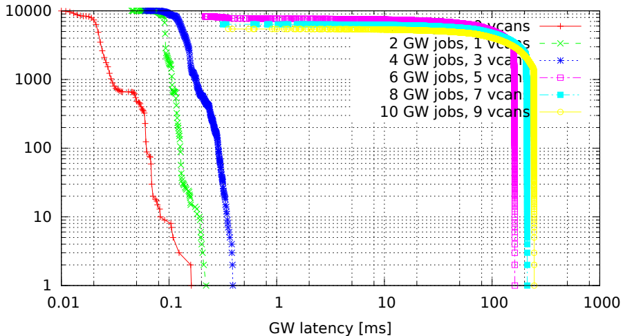
Chained GWs on multiple VCAN interfaces (GW kernel 2.6.33.7-00007-g9c0ff90, Traffic flood, Load none)
