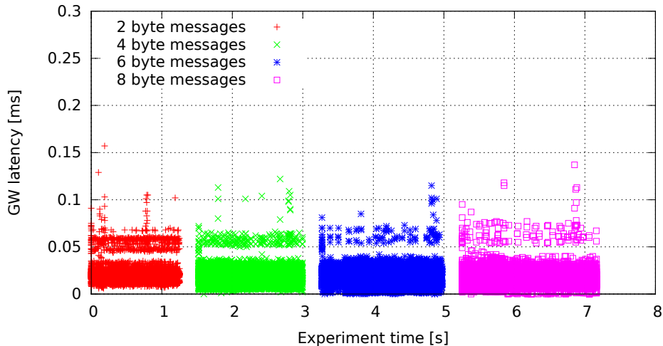
Single GW rule for all messages, no modifications (GW kernel 2.6.33.7-00007-g9c0ff90, Traffic flood, Load none)
