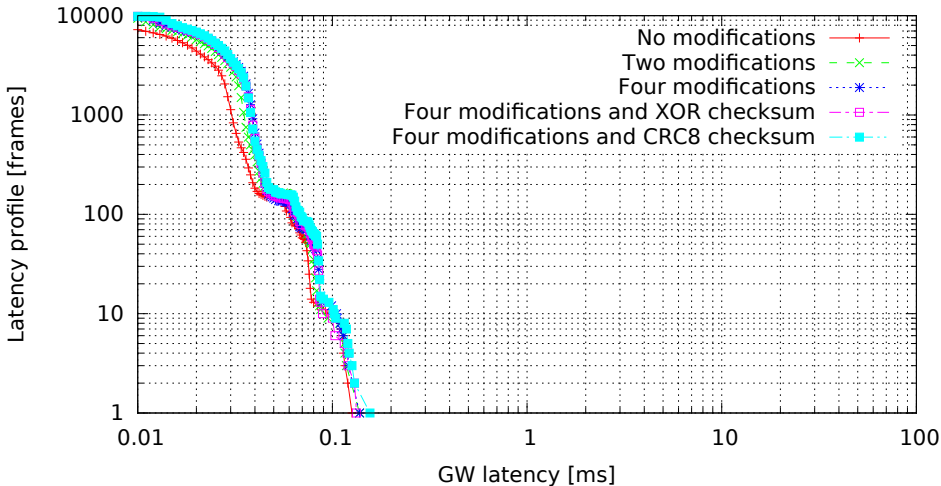
Single GW rule for all messages with modifications, 8 byte messages (GW kernel 2.6.33.7-00007-g9c0ff90, Traffic flood, Load none)
