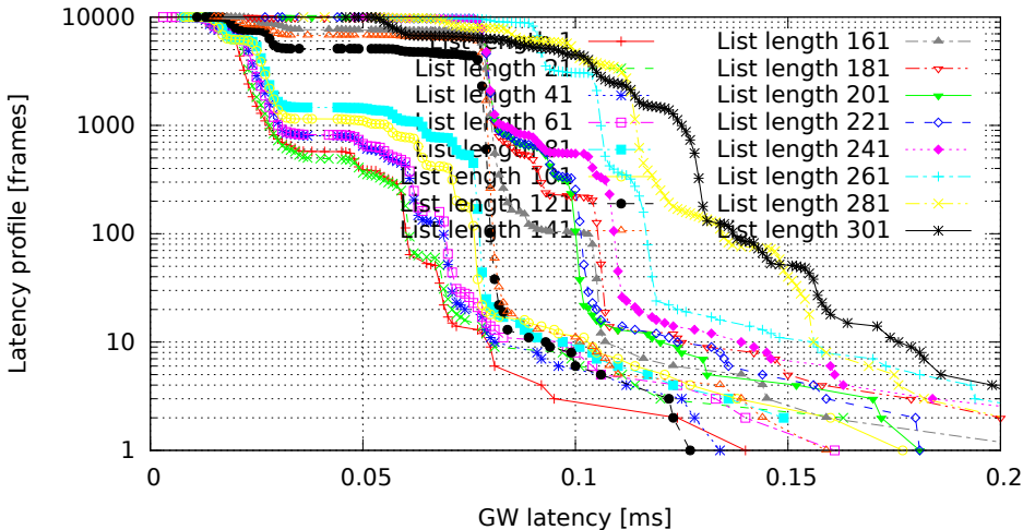
Different lengths of filter list, only the last one matches (GW kernel 2.6.33.7-00007-g9c0ff90, Traffic flood, Load none)
