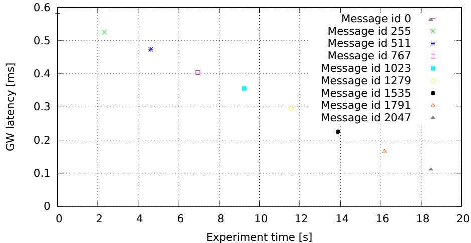
2048 GW rules (one per id, mask 0x7FF), no modifications (GW kernel 2.6.33.7-00007-g9c0ff90, Traffic flood, Load none)
