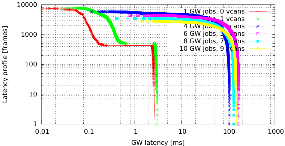
Chained GWs on multiple VCAN interfaces (GW kernel 2.6.33.7-00007-g9c0ff90, Traffic flood, Load eth)
