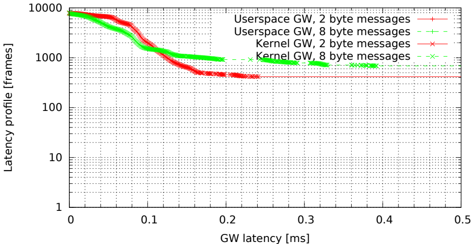
Kernel vs. userspace GW, no modifications (GW kernel 2.6.33.7-00007-g9c0ff90, Traffic flood, Load eth)
