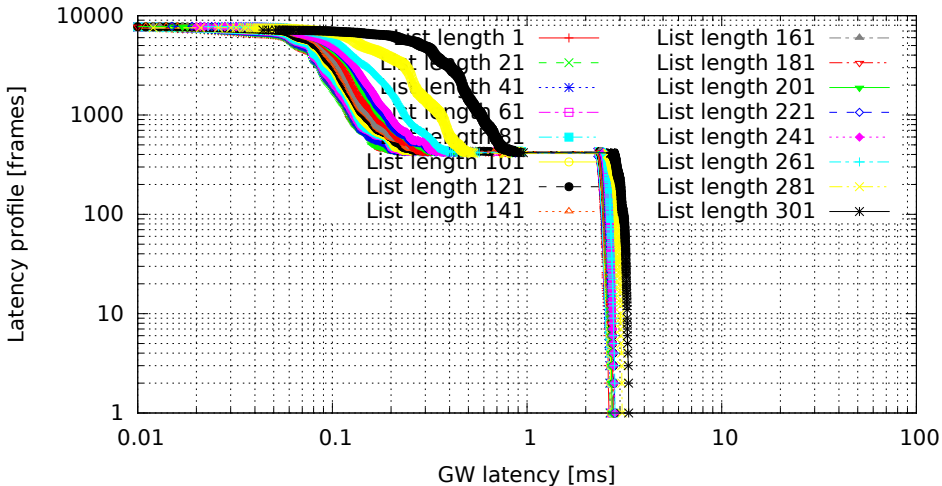
Different lengths of filter list, only the last one matches (GW kernel 2.6.33.7-00007-g9c0ff90, Traffic flood, Load eth)
