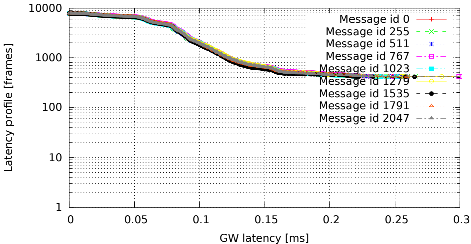
2048 GW rules (one per id, mask C00007FF), no modifications (GW kernel 2.6.33.7-00007-g9c0ff90, Traffic flood, Load eth)
