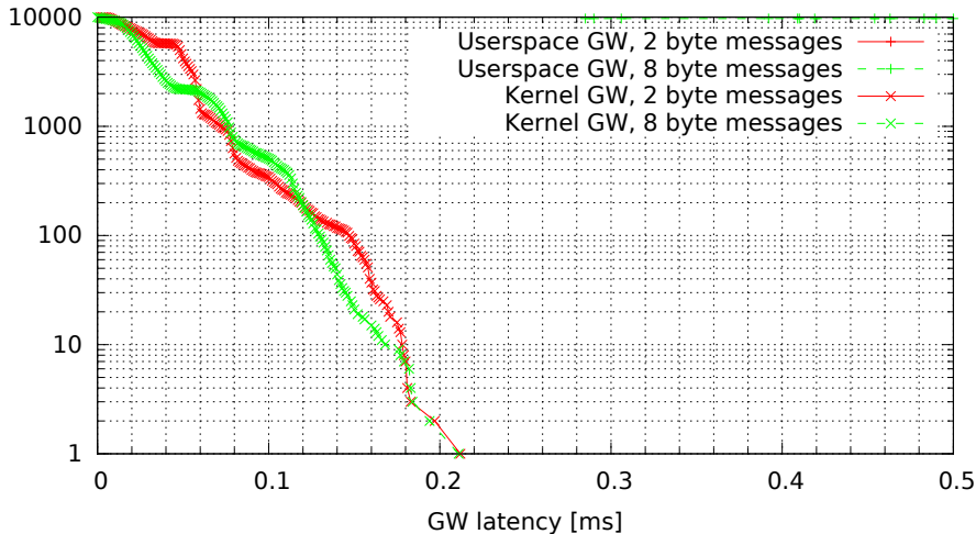
Kernel vs. userspace GW, no modifications (GW kernel 2.6.33.7-00007-g9c0ff90, Traffic flood, Load cpu)
