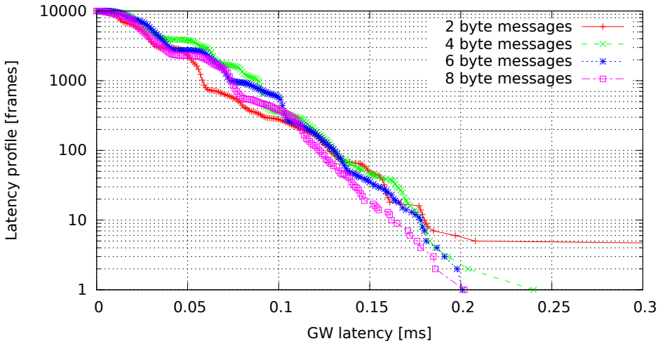
Single GW rule for all messages, no modifications, high (soft)irq task priority (GW kernel 2.6.33.7-00007-g9c0ff90, Traffic flood, Load cpu)
