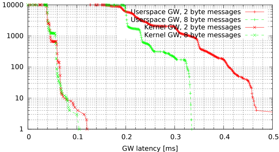
Kernel vs. userspace GW, no modifications (GW kernel 2.6.33.7-00007-g9c0ff90, Traffic 50, Load none)
