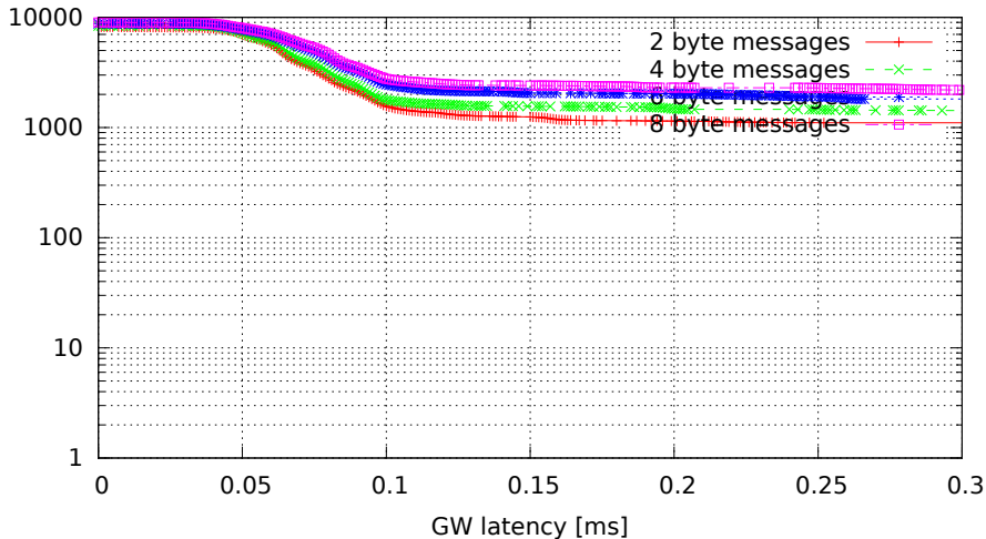
Single GW rule for all messages, no modifications, high (soft)irq task priority (GW kernel 2.6.33.7-00007-g9c0ff90, Traffic 50, Load eth)
