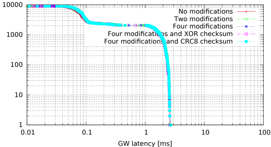
Single GW rule for all messages with modifications, 8 byte messages (GW kernel 2.6.33.7-00007-g9c0ff90, Traffic 50, Load eth)
