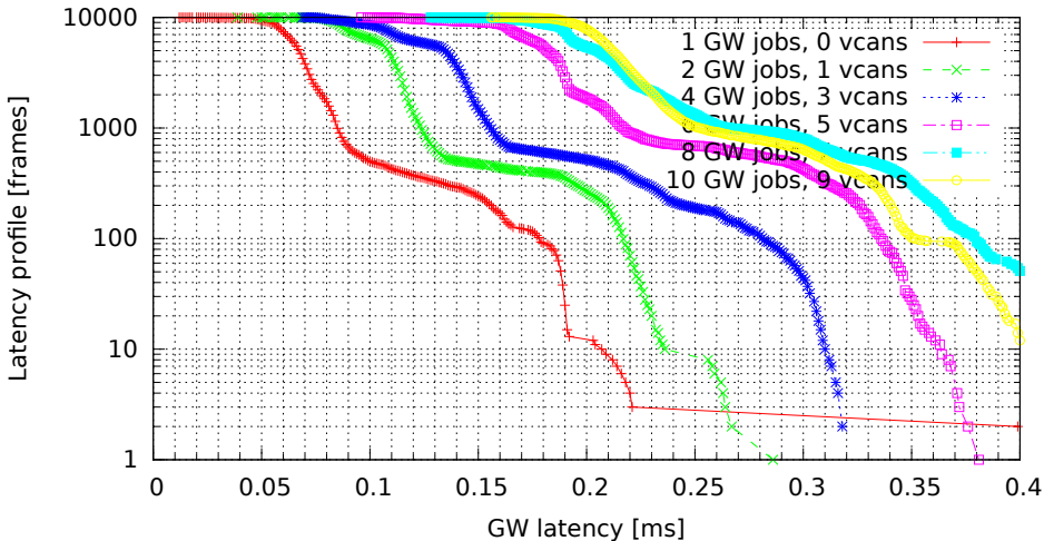
Chained GWs on multiple VCAN interfaces (GW kernel 2.6.33.7-00007-g9c0ff90, Traffic 50, Load cpu)
