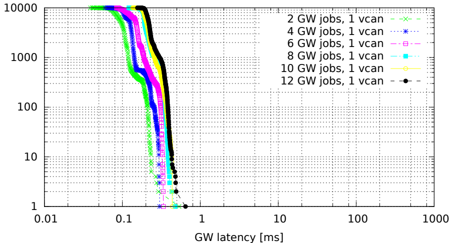
Chained GWs on a single VCAN interface (GW kernel 2.6.33.7-00007-g9c0ff90, Traffic 50, Load cpu)
