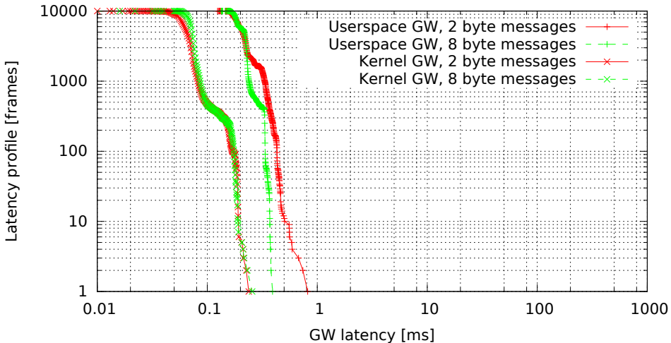
Kernel vs. userspace GW, no modifications (GW kernel 2.6.33.7-00007-g9c0ff90, Traffic 50, Load cpu)
