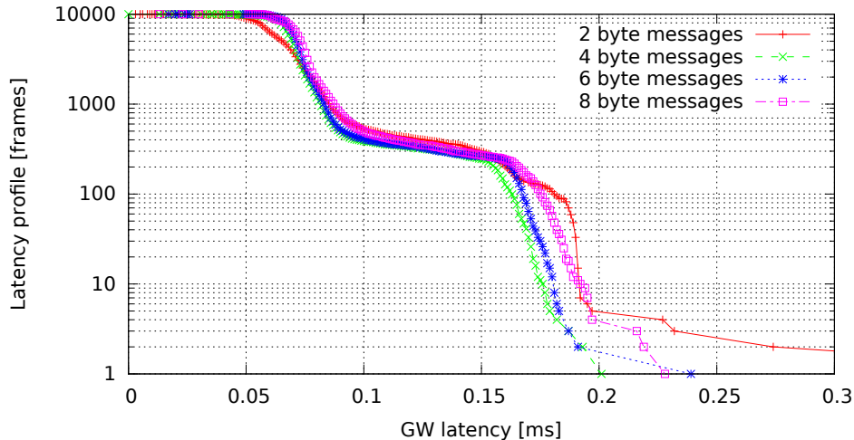
Single GW rule for all messages, no modifications (GW kernel 2.6.33.7-00007-g9c0ff90, Traffic 50, Load cpu)
