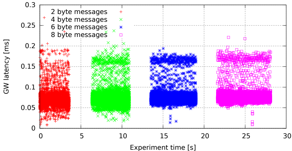
Single GW rule for all messages, no modifications, high (soft)irq task priority (GW kernel 2.6.33.7-00007-g9c0ff90, Traffic 50, Load cpu)
