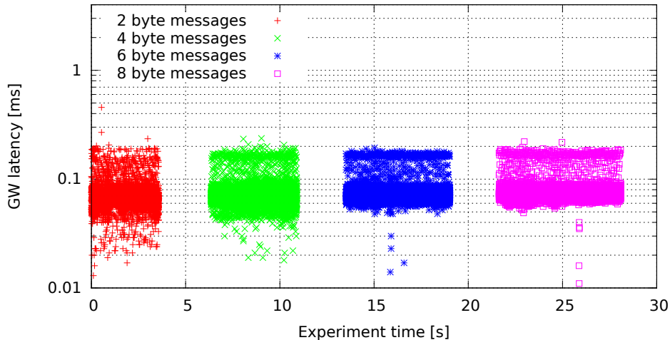
Single GW rule for all messages, no modifications, high (soft)irq task priority (GW kernel 2.6.33.7-00007-g9c0ff90, Traffic 50, Load cpu)
