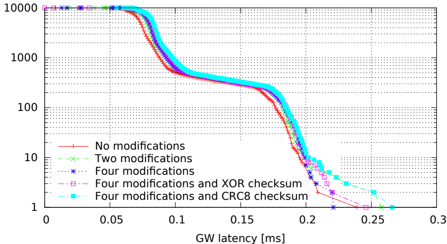
Single GW rule for all messages with modifications, 8 byte messages (GW kernel 2.6.33.7-00007-g9c0ff90, Traffic 50, Load cpu)
