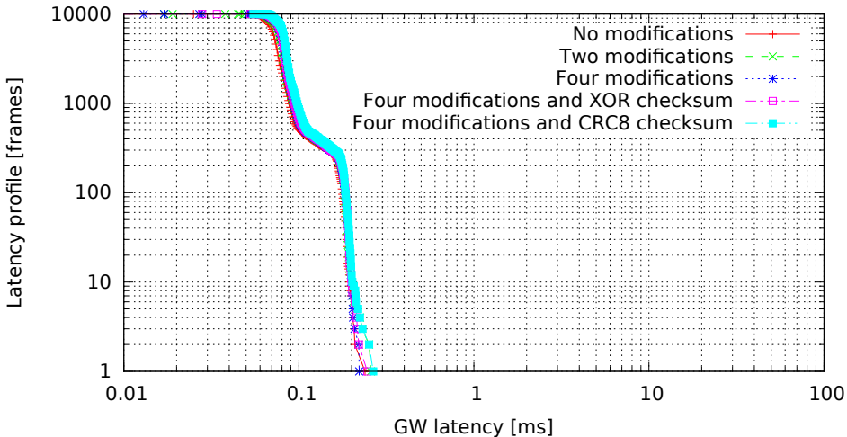
Single GW rule for all messages with modifications, 8 byte messages (GW kernel 2.6.33.7-00007-g9c0ff90, Traffic 50, Load cpu)
