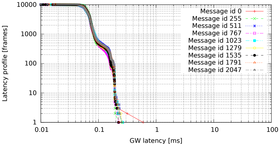
2048 GW rules (one per id, mask C00007FF), no modifications (GW kernel 2.6.33.7-00007-g9c0ff90, Traffic 50, Load cpu)
