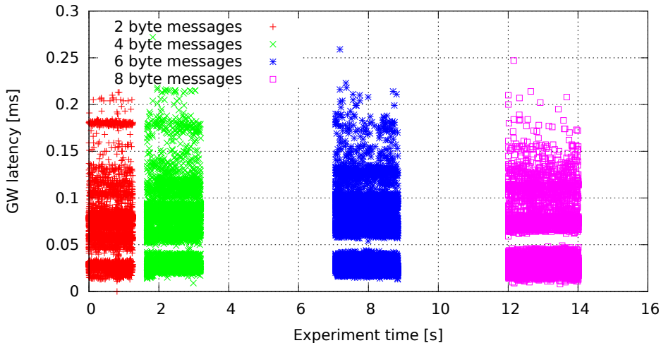
Single GW rule for all messages, no modifications, high (soft)irq task priority (GW kernel 3.0.4-00007-g1c8c373, Traffic flood, Load cpu)
